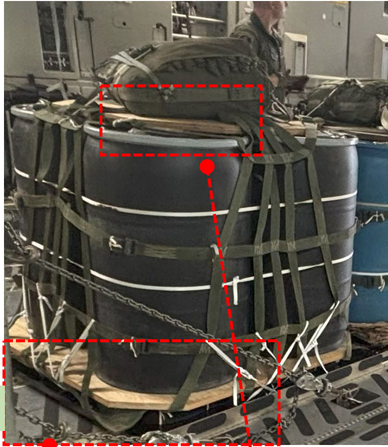
Figure 2 Zoomed Images of 3 Boards
