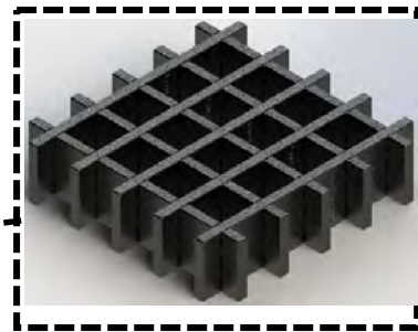
12x12x3" module REAL10M12
